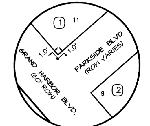
-BENCHMARK DETAIL- (LOCATED IN SECTION FOUR) 3" BRASS DISK SET IN A CONCRETE COLUMN 6" IN DIAMETER, THREE FEET DEEP AND BURIED FLUSH WITH NATURAL GROUND STAMPED: GH4 ELEVATION: 255.2
